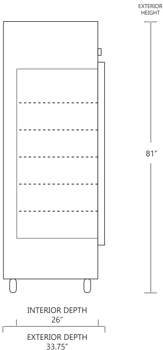
SIDE VIEW
